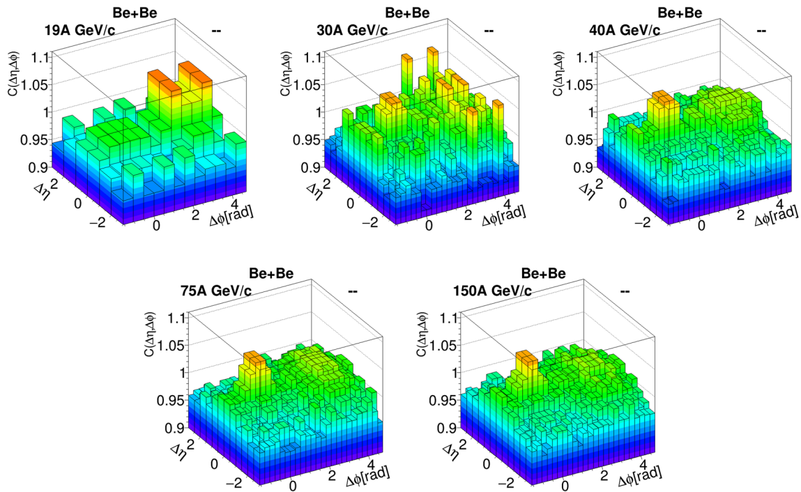
Fig. 9 Two-particle correlation function C(\Delta\eta, \Delta\phi) for negative charge pairs in the 5% most central Be + Be collisions at 19A–150A GeV/c
