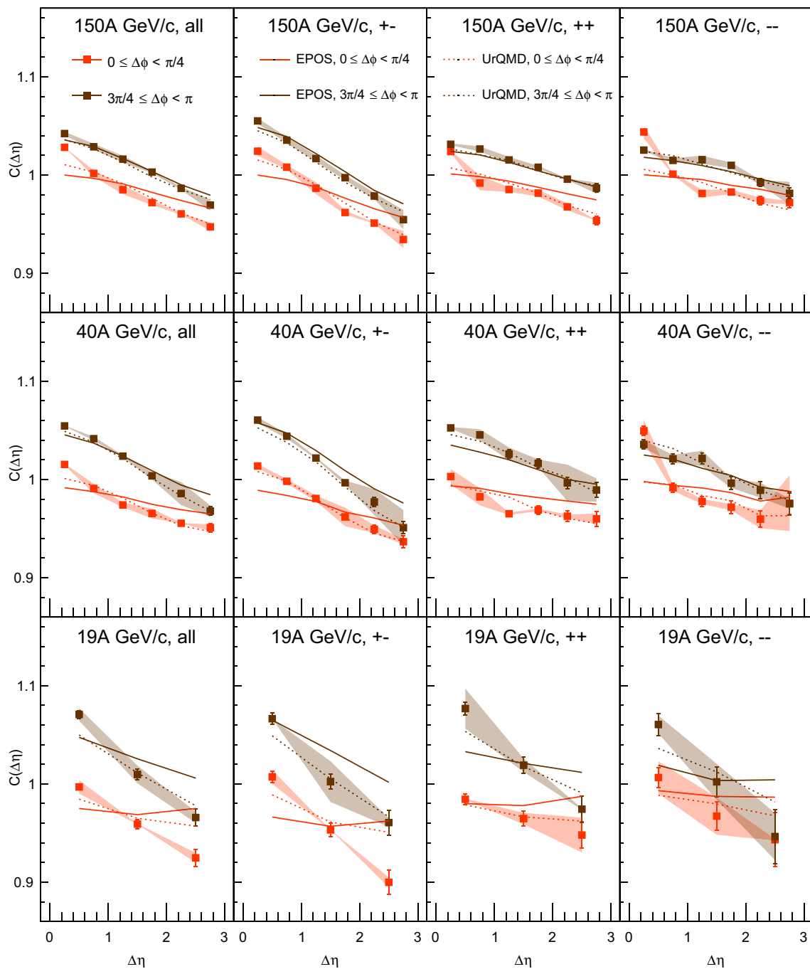
Fig. 16 Two-particle correlation function C(\Delta\eta) obtained from projection of C(\Delta\eta, \Delta\phi) onto the \Delta\eta axis for subranges of \Delta\phi . From left to right the columns show respectively: all charge pairs, unlike-sign pairs, positive charge pairs, and negative charge pairs. Vertical bars denote
