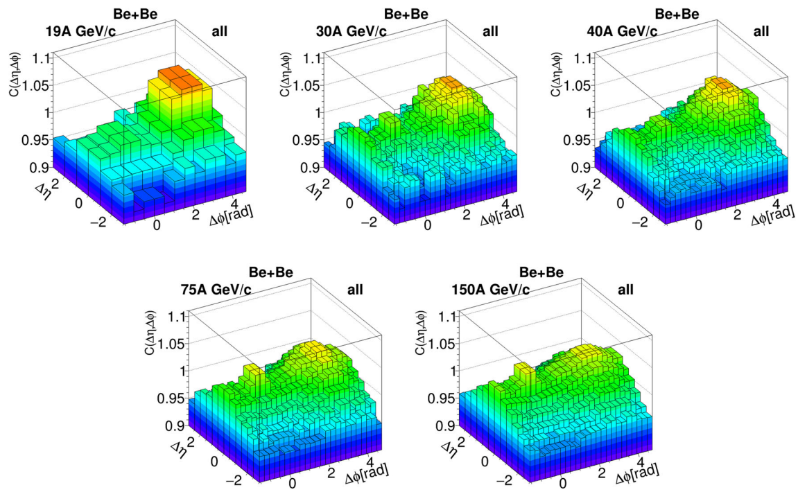
Fig. 6 Two-particle correlation function C(\Delta\eta, \Delta\phi) for all charge pairs in the 5% most central Be + Be collisions at 19A–150A GeV/c
