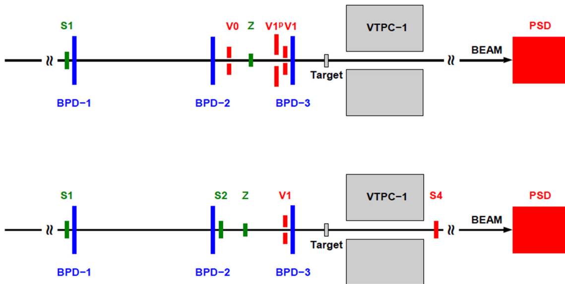
Fig. 2 The schematic of the placement of the beam and trigger detectors in high momentum ( top ) and low momentum ( bottom ) data taking
