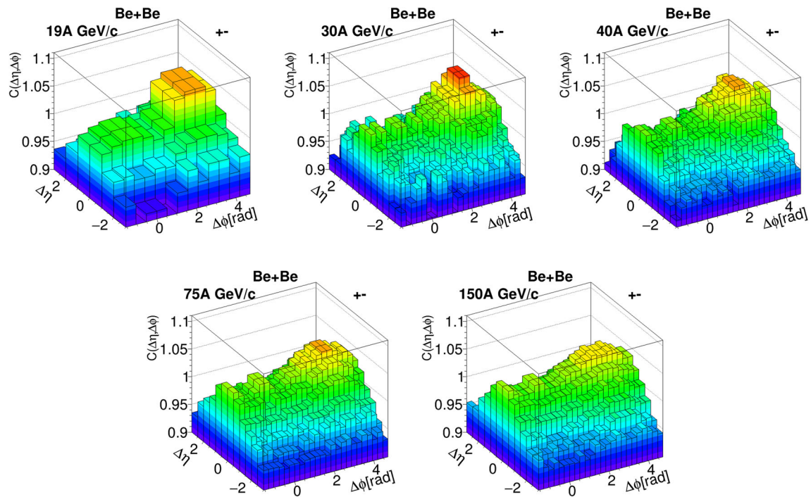
Fig. 7 Two-particle correlation function C(\Delta\eta, \Delta\phi) for unlike-sign pairs in the 5% most central Be + Be collisions at 19A–150A GeV/c
