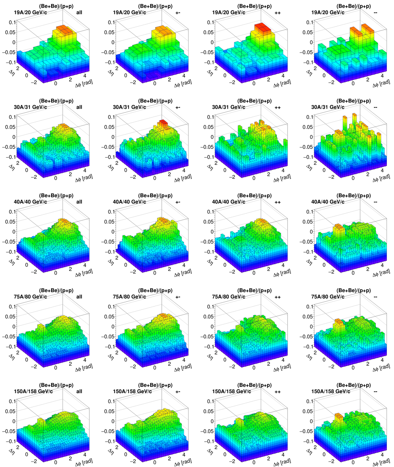
Fig. 11 Ratio R_{pp}^{BeBe} for all pair combinations and momenta (following formula Eq. 4). Each row shows different beam momentum (beam momentum increases downwards). Every column presents results for
