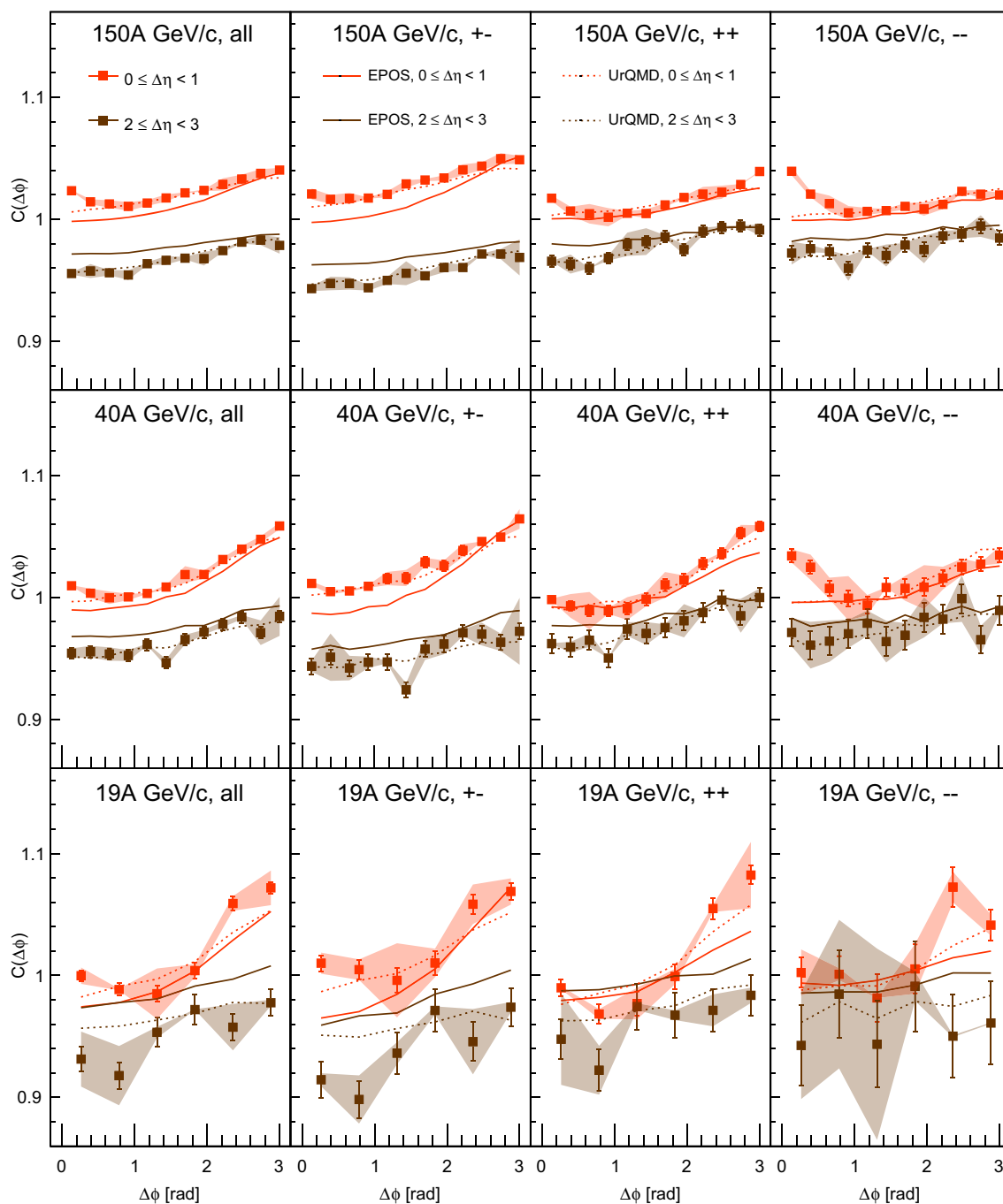
Fig. 17 Two-particle correlation function C(\Delta\phi) obtained from projection of C(\Delta\eta, \Delta\phi) onto the \Delta\phi axis for subranges of \Delta\eta . From left to right the columns show respectively: all charge pairs, unlike-sign pairs, positive charge pairs, and negative charge pairs. Vertical bars denote
