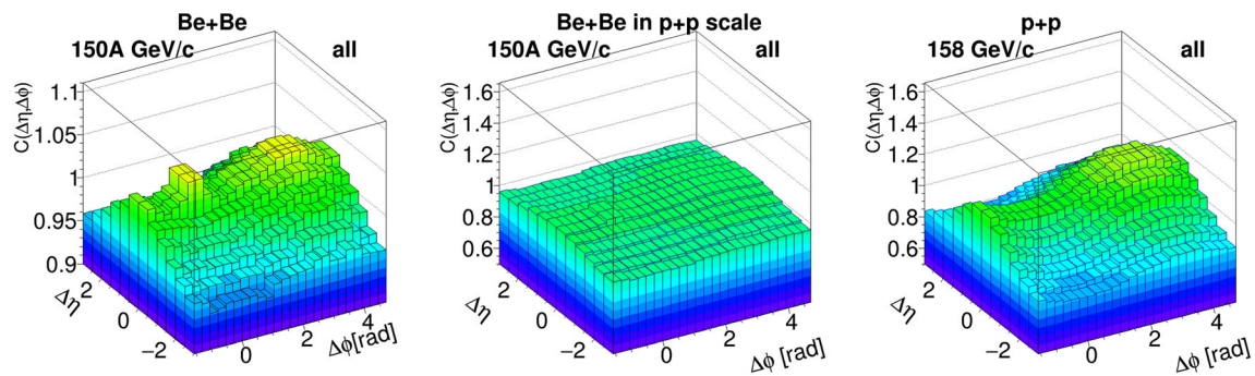
Fig. 10 Comparison of correlation functions C(\Delta\phi) for the 5% most central Be + Be collisions and inelastic p + p interactions. Left column shows the correlation function for all charge pairs in Be + Be collisions at beam momentum 150A GeV/c per nucleon. Middle column: the same
