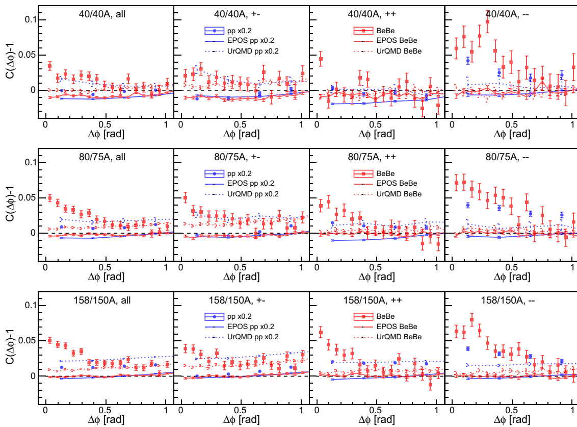
Fig. 13 Comparison of two-particle correlation function C - 1 for the range \Delta\eta \in [0, 0.5) and for zoomed in range of 0 \leq \Delta\phi \leq 1 radians. Results of collisions of p + p are marked in blue and of Be + Be are marked in red. Columns from left to right show results for: all charge pairs, unlike-sign pairs, positive pairs, and negative pairs. Results for beam momenta 40A, 75A, and 150A GeV/c are plotted in successive
