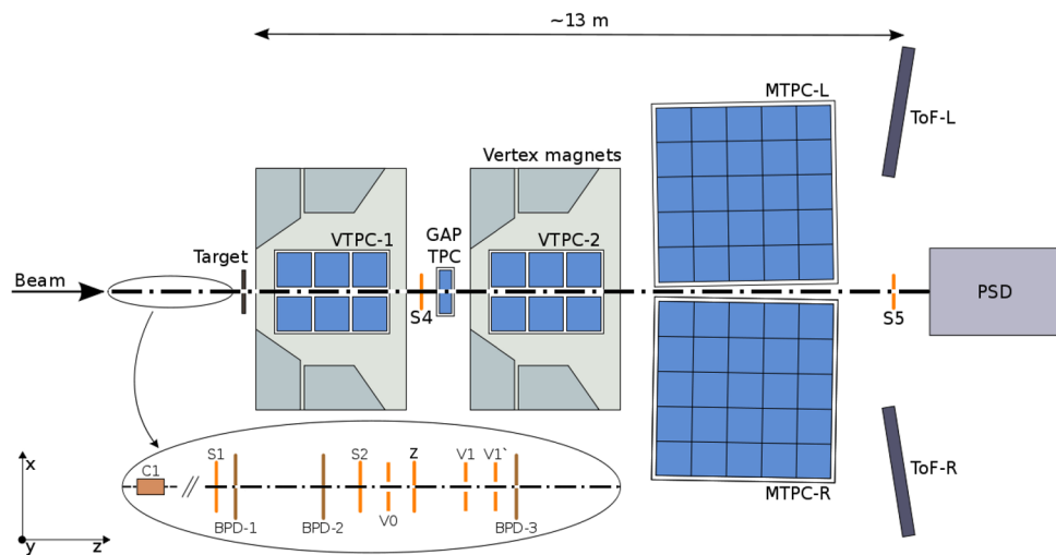
Fig. 1 The schematic layout of the NA61/SHINE experiment at the CERN SPS [1] showing the components used for the Be + Be energy scan (horizontal cut, not to scale). The beam instrumentation is sketched in the inset. Alignment of the chosen coordinate system as shown in the
