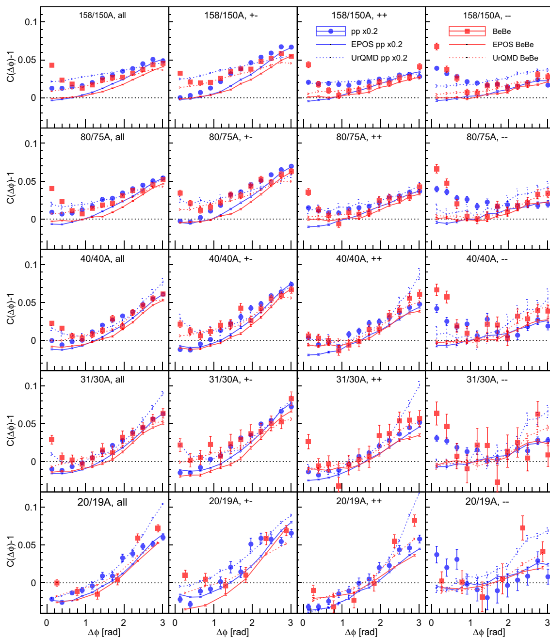
Fig. 12 Comparison of two-particle correlation function C - 1 for the range \Delta\eta \in [0, 0.5) in collisions of p + p (blue) and Be + Be (red). Columns from left to right show results for: all charge pairs, unlike-sign pairs, positive pairs, and negative pairs. Results for different beam momenta are plotted in successive rows. Data results are shown by
