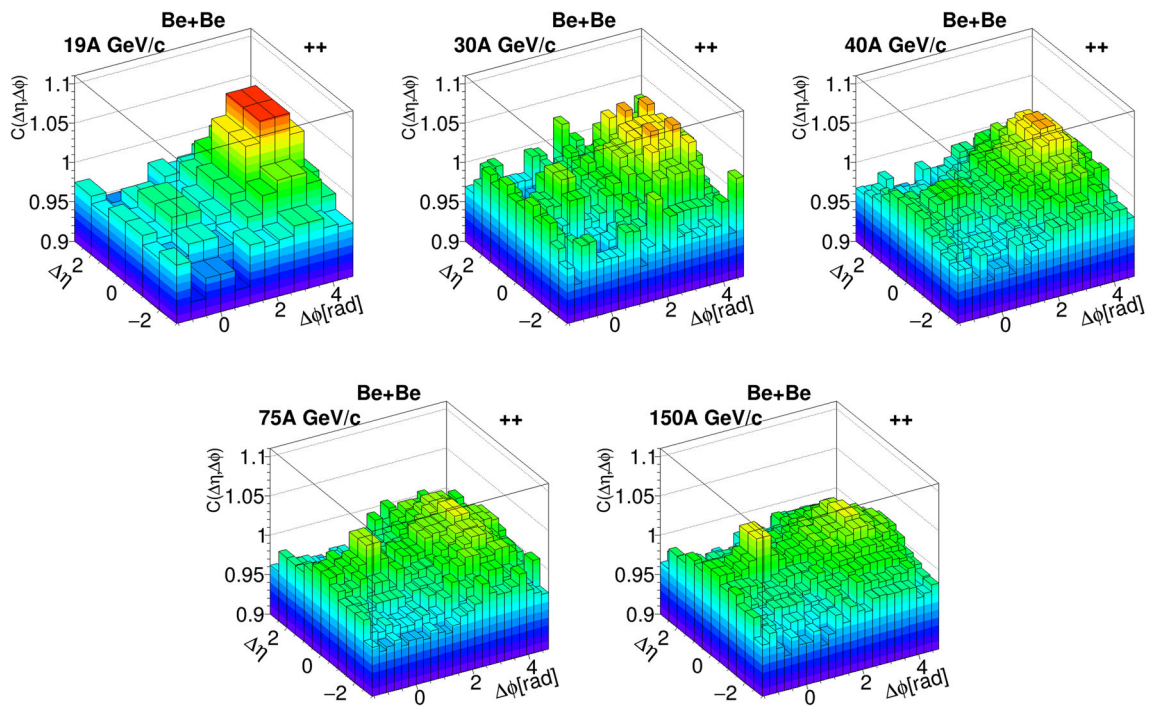
Fig. 8 Two-particle correlation function C(\Delta\eta, \Delta\phi) for positive charge pairs in the 5% most central Be + Be collisions at 19A–150A GeV/c
