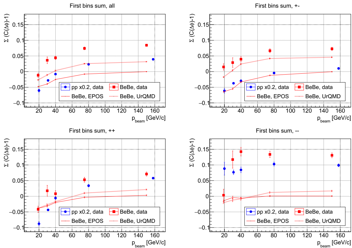
Fig. 15 The sum of two-particle correlation function C(\Delta\eta, \Delta\phi) in the \Delta\phi region [0, \pi/2) and \Delta\eta \in [0, 0.5) for different charge combinations. Top left picture for all charge pairs, top right for unlike-sign, bottom left for positive charged pairs, bottom right for negative charged.
