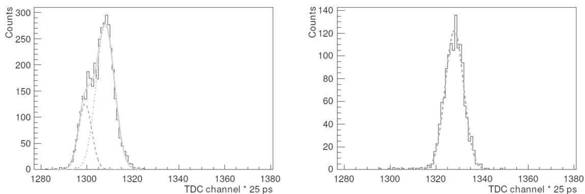
Fig. 4 Time-of-flight of fragments of Z/A with momentum of 13.9 GeV/c. Left: carbon ions shows double Gaussian structure due to two isotopes of carbon in the beam. Right: beryllium ions show single Gaussian distribution, indicating isotopic purity of the beryllium in the beam
